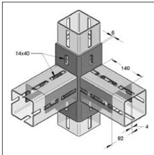
CENTUM® Winkelverbinder 90°
